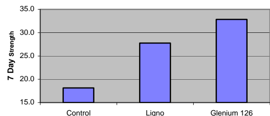
Compressive Strength @ 1.0% Dosage @ S4 (180 slump)
